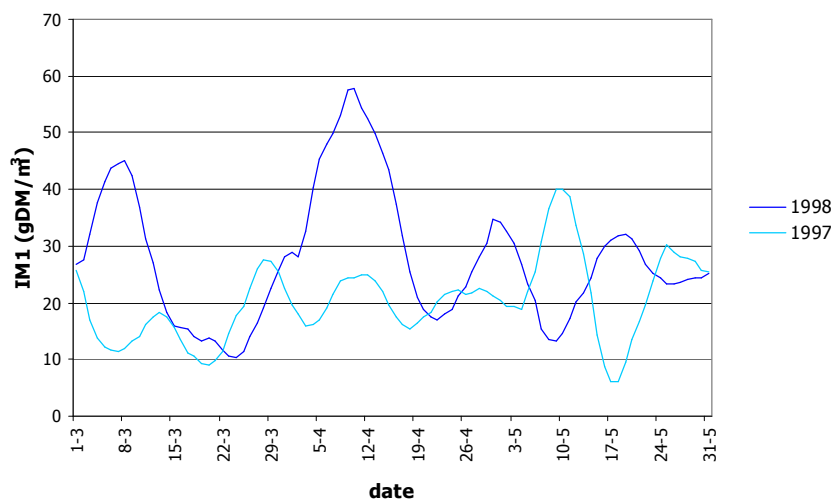
Figure 4.18 Modelled background silt concentration IM1 (moving average over a period of 7 days) during spring in 1997 and 1998 [model results WL | Delft Hydraulics]
